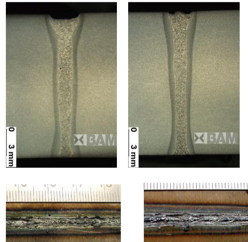
Fig. 7: Positional welding PF (up) 90°, t = 16 mm
