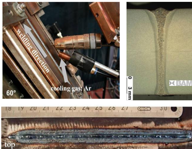
Fig. 6: Positional welding PF (up) 60°, t = 16 mm
